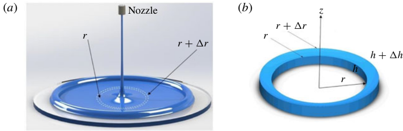
FIGURE 2. (a) Schematic of the liquid film and hydraulic jump created by an impinging jet. (b) Control volume of the film element on which the energy balance is applied.
