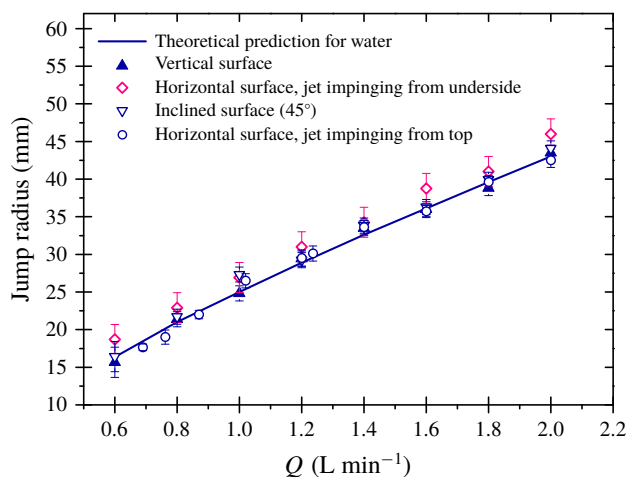
FIGURE 4. Jump radius plotted against jet flow rate for the four surface orientations. In each case the liquid was pure water. The theoretical prediction (line) is obtained ignoring gravity by setting g = 0 in (5.6).
